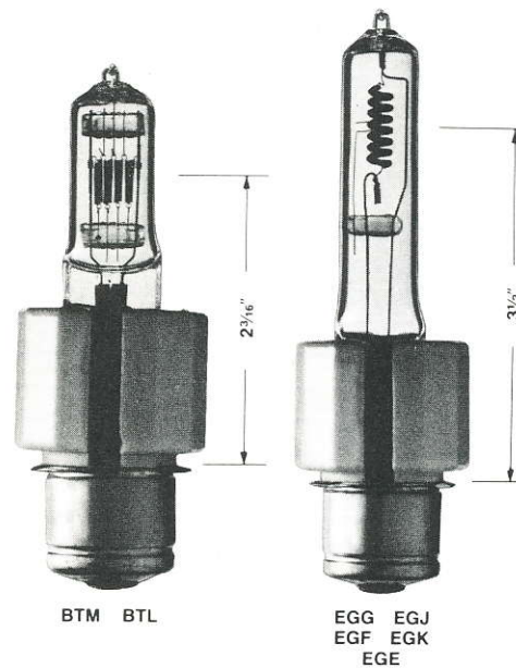
MEDIUM PREFOCUS LAMPS WITH 2 3/16" LCL (P28s) MEDIUM PREFOCUS LAMPS WITH 3 1/2" LCL (P28s)
