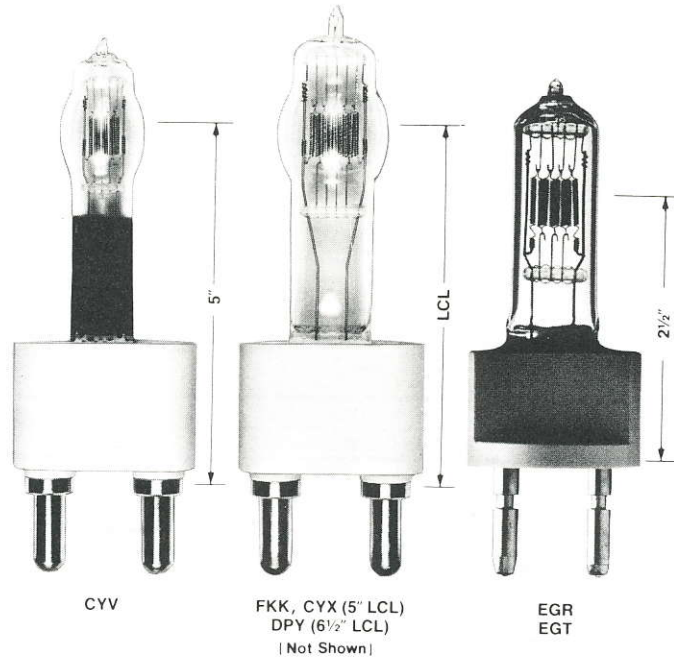
MOGUL BIPOST LAMPS WITH 5" AND 6 1/2" LCL (G 38) MEDIUM BIPOST LAMPS WITH 2 1/2" LCL (G 22)
