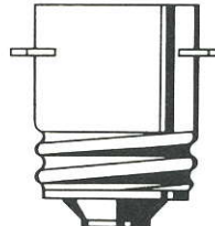
P40s DIN: 49728 IEC: 7004-43 ANSI: Mogul prefocus base
